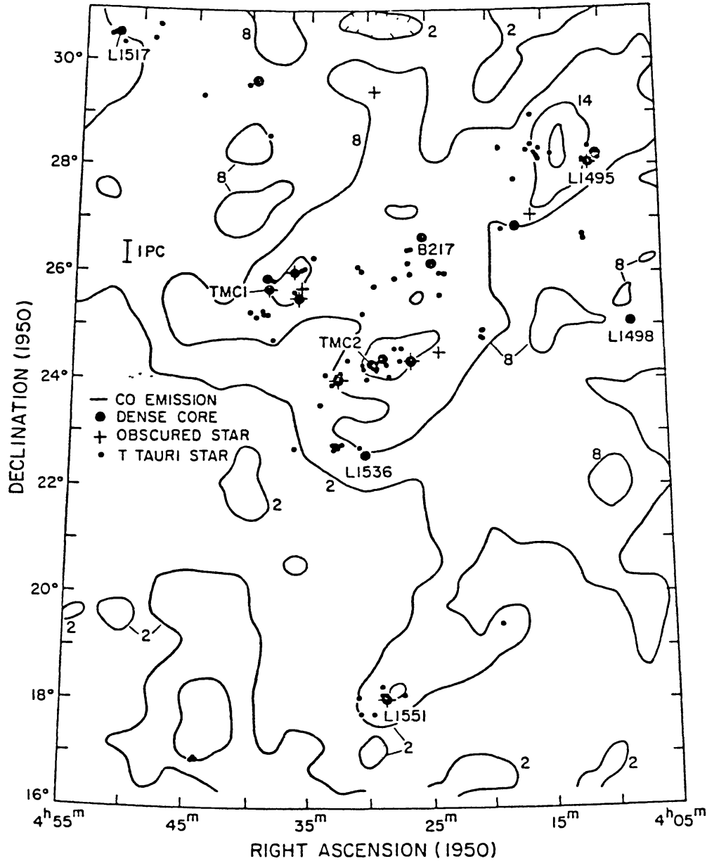
Figure 2 CO contour map of the Taurus molecular cloud with positions of dense \text{NH}_3 cores, embedded infrared sources, and visible T Tauri stars (from Myers 1986).
