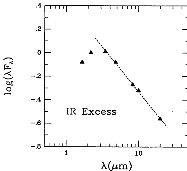
Figure 6 Composite spectral energy distribution of nine T Tauri stars. The dashed line shows that the near- and mid-infrared excess is well represented as a power-law spectrum with index n = 0.75 . A stellar blackbody would give n = 3 (from Rydgren & Zak 1987).
